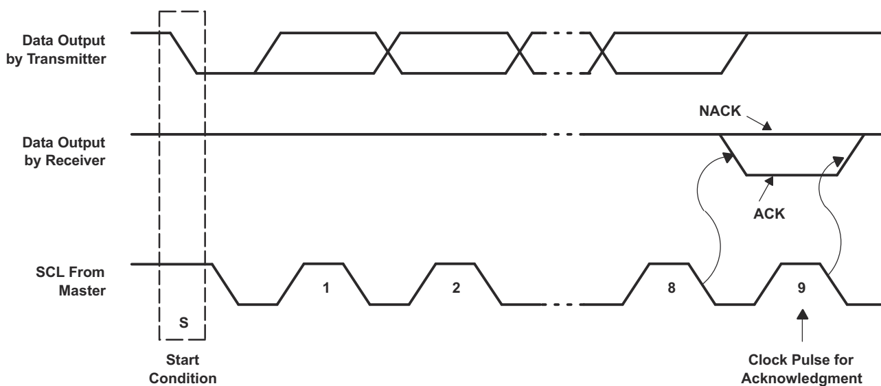
图 8-3. Acknowledgment on I²C Bus
