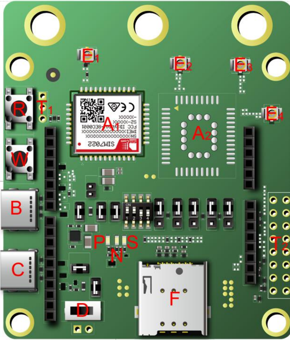
Figure 1: The top view of NB-EVB
