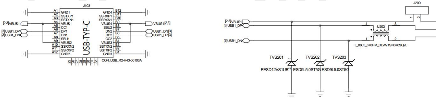
Figure 10: The reference design of USB to UART
