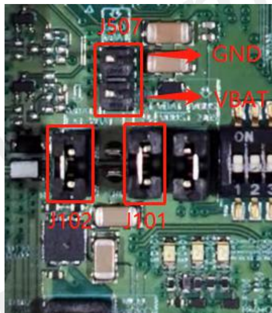
Figure 16: Jumpers J101 J102 and J507
