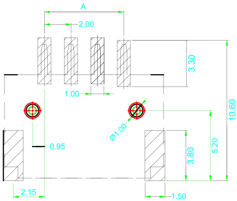
P. C. B LAYOUT
